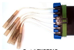
Part # TXOTC67 Diesel Injector Connector Harness for Ohm Testing for Dodge/Cummins 5.9L & 6.7L 2006-2014
