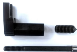
Part # TX67F-T Diesel Fuel Injector Removal Tool- 2010-2015 Ford Powerstroke 6.7L
