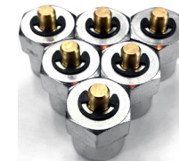
Part # TX59CT-6 Diesel Injector Cap/Block-Off Tool Set 5.9L Dodge/Cummins (Set of 6)
